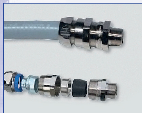
Anaconda Exe/d Kabel-Schlauchverschraubung Anaconda Exe/d cable-hose-fitting Anaconda Exe/d raccord presse-étoupe
