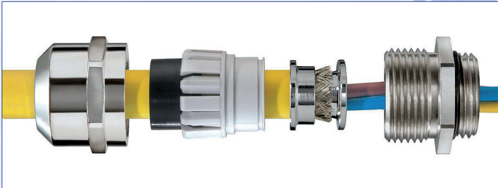
Wiska Sprint Exe EMV Messing vernickelt Wiska Sprint Exe EMV nickel plated brass Wiska Sprint Exe EMV laiton nickelé
